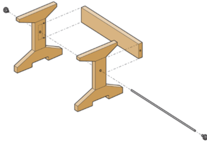
Trestle Construction
