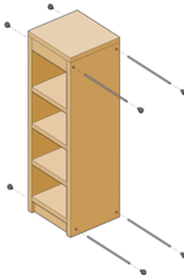
Carcass Construction
